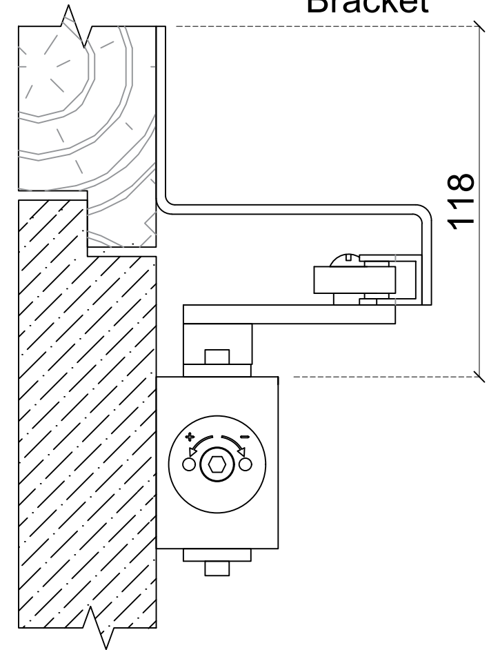
Push Open with Rebated Over Panel Bracket
